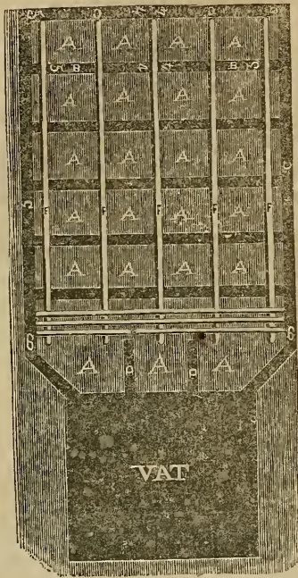
Fig. 3. Platform or ground plan, where the ground is level and without excavation, with the lye vat.
